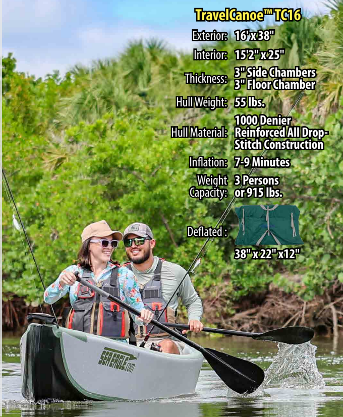
Rigid bow and stern molds provide clean entry and clean exit and they roll up easily with the canoe when deflated.
